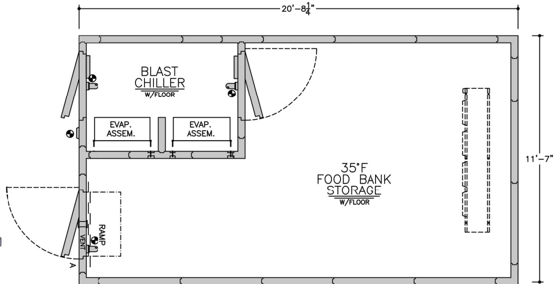
Fig. 2 - Large food bank with double depth blast chiller compartment
