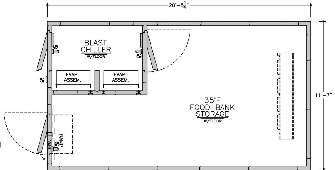
Fig. 2 - Large food bank with double depth blast chiller compartment
